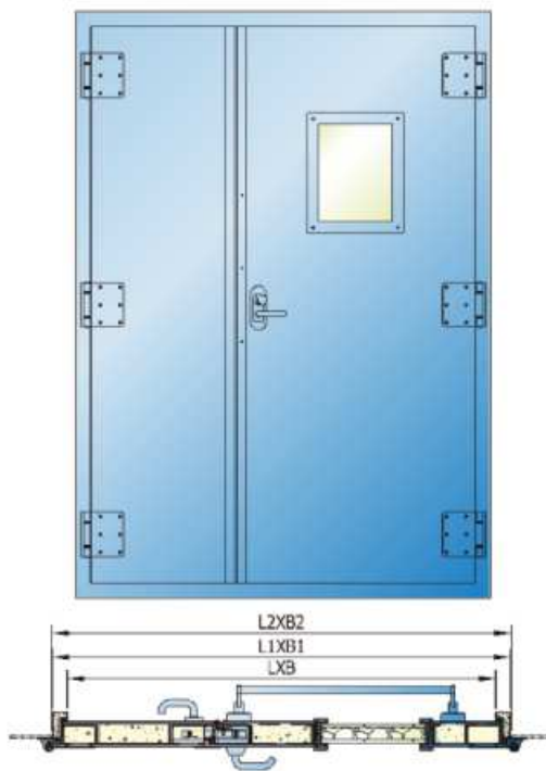
262WHL651C-00 DOUBLE-LEAF
