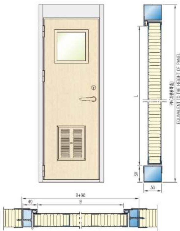
262WHL006S-00 B15 CLASS PANEL INSTALLED DOOR
