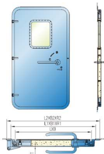
A60 QUICK ACTION WEATHERTIGHT STEEL DOOR (SINGLE)
