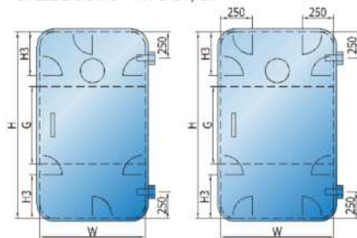
STEEL DOOR OF TYPE BY, CY
