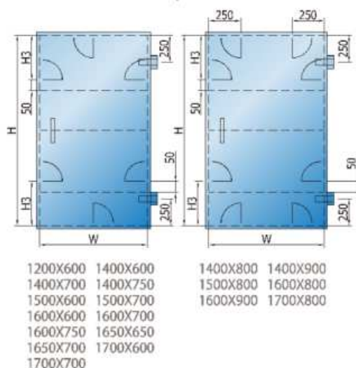
STEEL DOOR OF TYPE AF,AY
