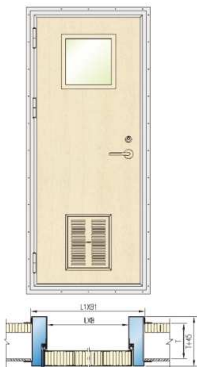
262WHL006X-00 B15 CLASS FIRE-PROOF DOOR
