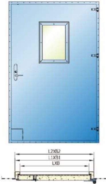
262WHL653-00 SINGLE-LEAF
