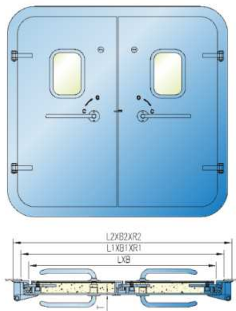
A60 QUICK ACTION WEATHERTIGHT STEEL DOOR (DOUBLE)
