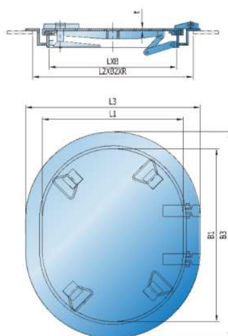
TYPE B ELLIPTIC
