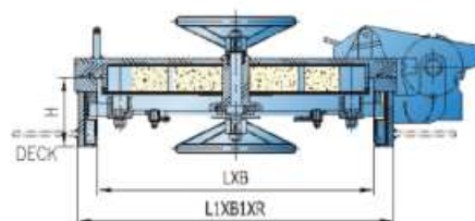
TYPE B HORIZONTAL INSTALLED ON DECK
