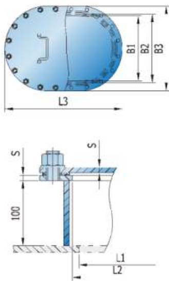
TYPE B MANHOLE COVER
