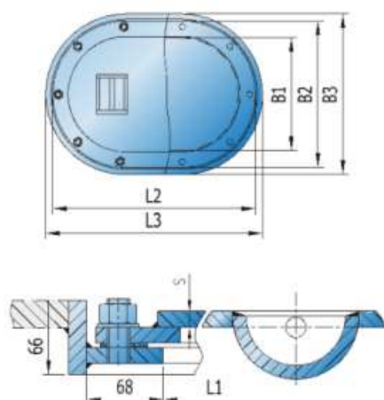
TYPE D MANHOLE COVER
