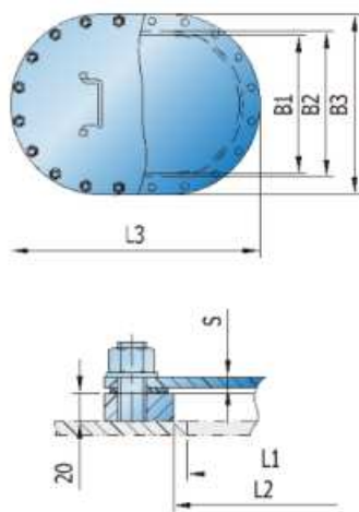
TYPE B MANHOLE COVER
