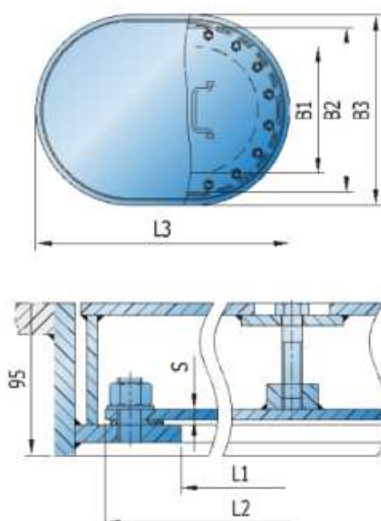
TYPE C MANHOLE COVER
