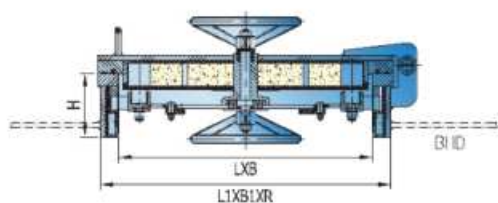
TYPE A VERTICALLY INSTALLED ON BULKHEAD
